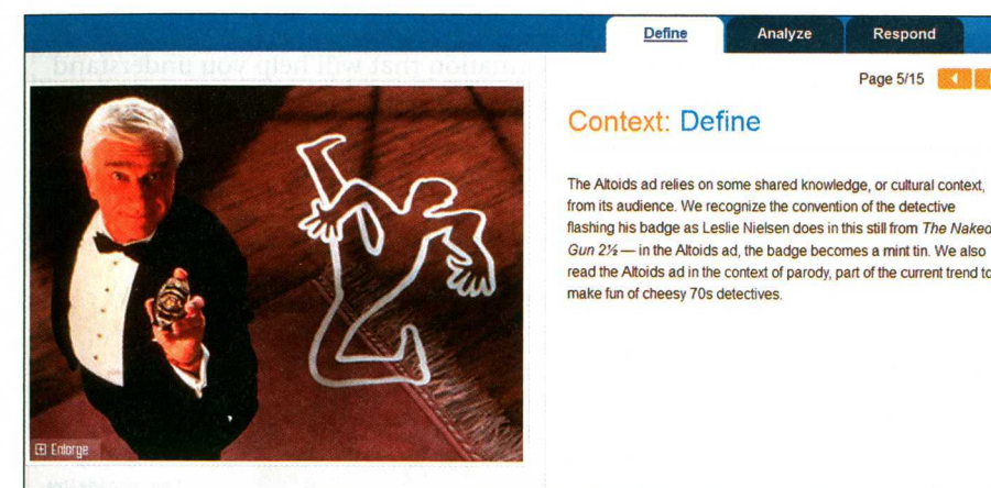
Figure 2.5 ix: visualizing composition: Context
