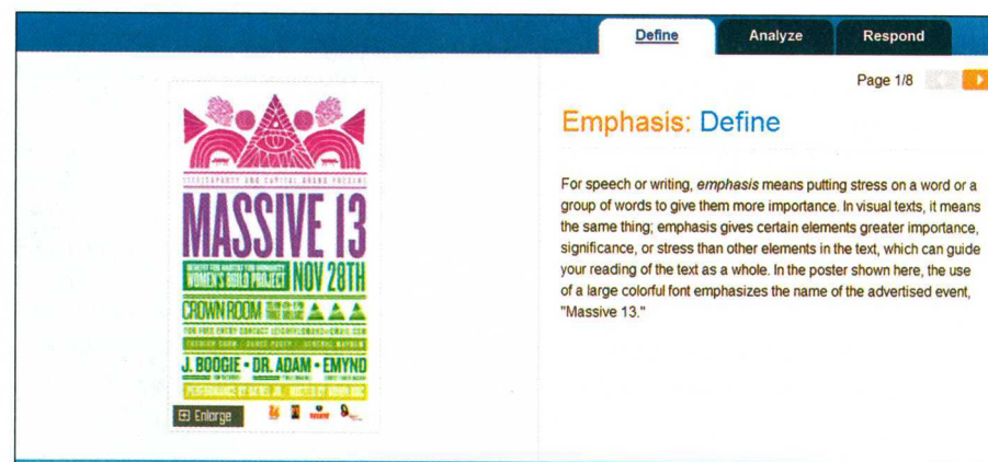
Figure 2.11 ix: visualizing composition: Emphasis
